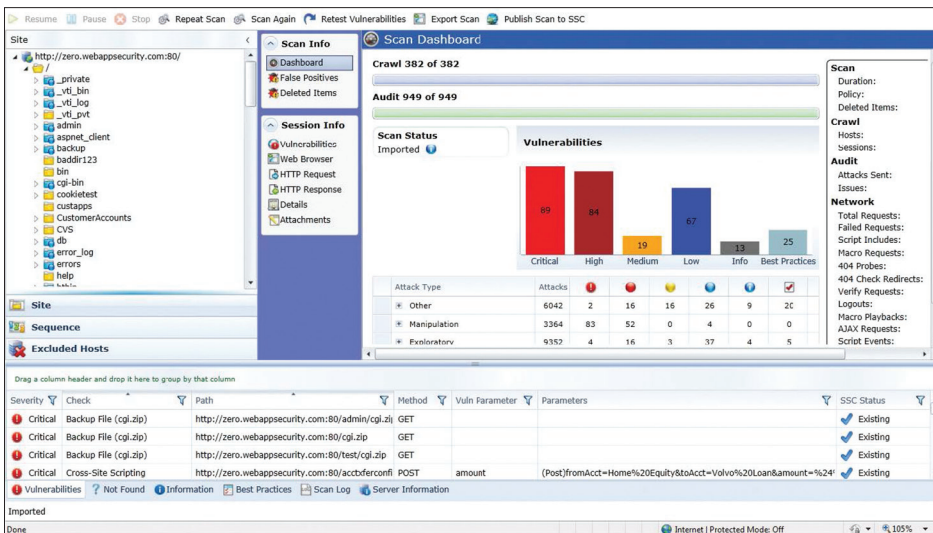
Figure 2. The Web-based GUI of WebInspect Enterprise
